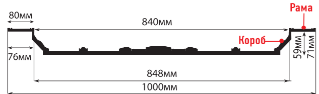
КР100-18D (1000x1000x71) рама: 1000x1000x12 короб: 848x848x59
