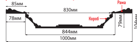
КР100-43 (1000x1000x104) рама: 1000x1000x25 короб: 844x844x79
