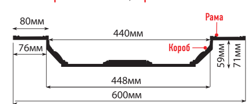
KS61-19D рама: 600x600x12, короб: 448x448x59
