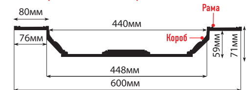
KS61-57 рама: 600x600x12, короб: 448x448x59
