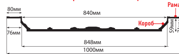
KP100-58 (1000x1000x71) рама: 1000x1000x12 короб: 848x848x59
